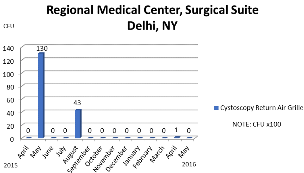
Chart 'B6': Cystoscopy Return Air Grille
