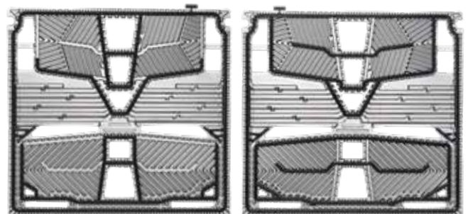
Alfa Laval AQUA process plate
