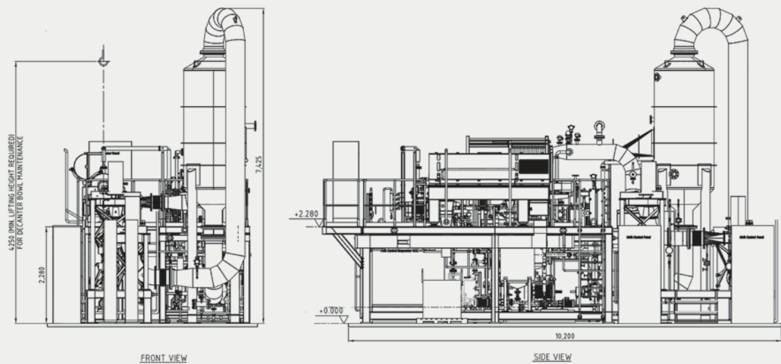
AlfaFlash ZLD MVR-D 1E-2.5 main dimensions
