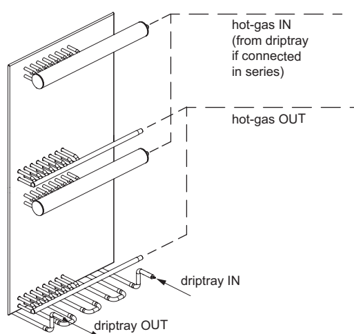
ISB pumped, bottom feed, 4 connections
