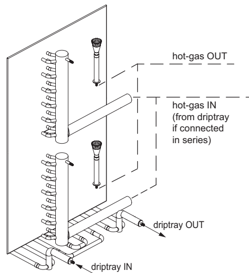
ISB direct expansion, 4 connections
