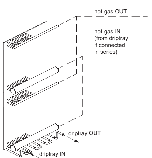
ISB pumped, top feed, 4 connections
