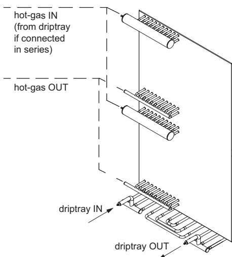
ISD pumped, top feed, 4 connections
